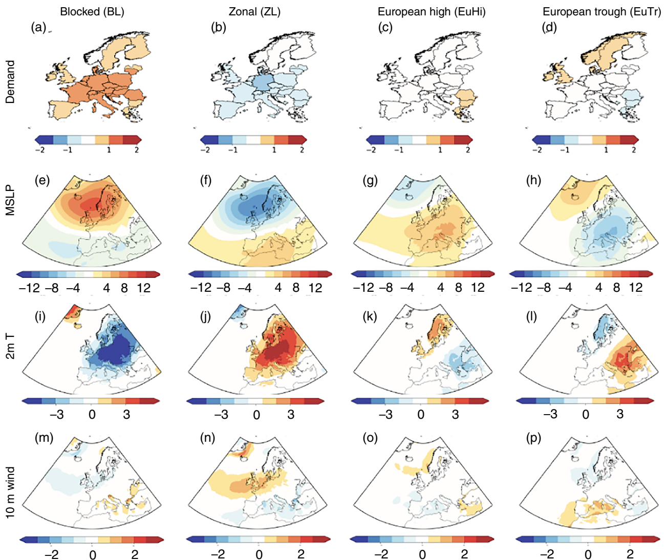
FIGURE 3 Surface response to each of the four targeted circulation types (TCTs) (columns) constructed using normalized demand, expressed as anomalies with respect to climatology (November–March). Row 1 shows normalized demand (units correspond to SD of each country’s anomaly time series; see Figure 1 and the discussion in Section 2.5). Rows 2–5 show mean sea level pressure (MSLP) (hPa), 2 m temperature (K) and 10 m wind speed ( \text{m}\cdot\text{s}^{-1} ), respectively
