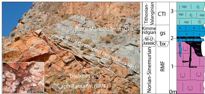
Figure 3. Triassic-Jurassic carbonate succession at Spinasanta quarry. The Upper Triassic-Lower Jurassic peritidal limestones of the Capo Rama Fm (RMF) are dislocated by synsedimentary faults. The Jurassic red bauxite clays (bx) fill erosional ponds at the top of the RMF and a dense network of neptunian dykes (inset). Kimmeridgian dasycladacean and gasteropods limestone (gs) and Upper Tithonian-Valanginian Pizzo Manolfo limestone (CTI), onlap the older strata.
