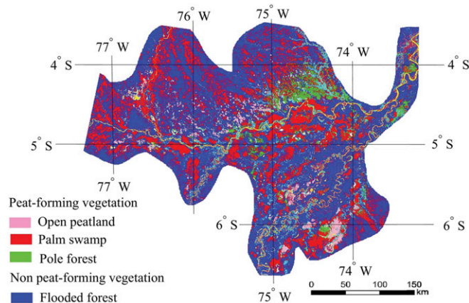
Fig. 1. Distribution of peat-forming and non-peat-forming vegetation in the PMFB at the resolution of 90 × 90 m (13). The map was resized to 1.69 × 1.69 km. Colors represent vegetation types: open peatland (pink), PS (red), PF (green), and FF (dark blue). Yellow represents open water, and light blue represents other. See figures 1 and 4 of ref. 13 for the original map.
