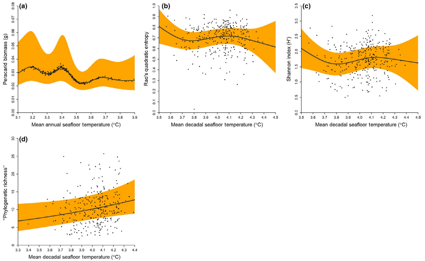
FIGURE A13 Partial relationships between mean annual/decadal sea floor temperature ( ^{\circ}\text{C} ) at sampling locations ( n = 312 ) in the Northwest Atlantic Ocean and different metrics of the biodiversity of peracarid assemblages sampled. Solid lines are smoothed lines of best fit as determined by multivariate generalized additive modeling. Colored bands are 95% confidence intervals. (a) Mean annual temperature/peracarid biomass; (b) mean decadal temperature/Rao's quadratic entropy; (c) mean decadal temperature/Shannon Index; (d) mean decadal temperature/phylogenetic richness
