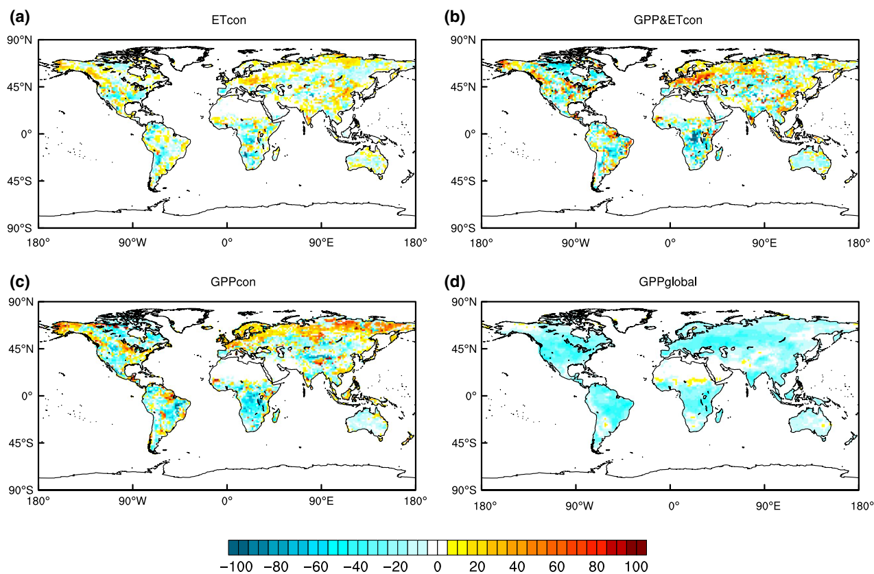
Fig. 4 Effect of the different constraints on the future change in GPP_{\max} ( gC\ m^{-2}\ month^{-1} ). The effect is defined as the difference in the future change (2084–2100 minus 1989–2005) in GPP_{\max} between the prior and the constrained ensembles. Positive values indicate higher increase in future GPP in the constrained ensemble compared to the prior ensemble.
