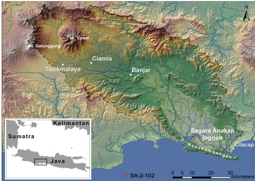
FIGURE 1 Map of the Segara Anakan Lagoon and its catchment area. The Segara Anakan Lagoon's watershed is marked with dashed lines
