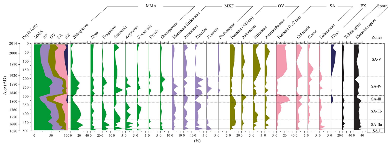
FIGURE 3 Pollen diagram of the Segara Anakan Lagoon core. Pollen were classified into five groups as follows: MMA: mangrove and mangrove associate; MXF: mixed forest; OV: open vegetation; SA: staple agriculture; and EX: exotic species. Selected taxa are shown. Complete list of taxa is provided in Supplementary S1
