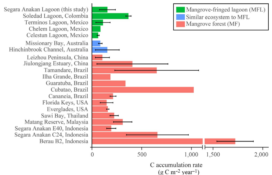
FIGURE 8 Comparison of C accumulation rates of mangrove-fringed lagoons and similar ecosystems and of mangrove forests. Extended information regarding the datasets included in the analysis is provided in Table 4
