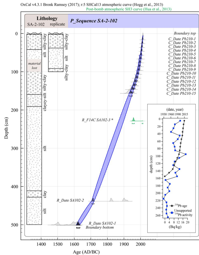
FIGURE 2 Lithology and age–depth model of cores taken from the Segara Anakan Lagoon. The age–depth model was constructed using the P-sequence in OxCal v 4.3.1 (Ramsey, 2009) and the initial ShCal.13 and PostBomb calibration curves (Hogg et al., 2013; Hua, Barbetti, & Rakowski, 2013). The unsupported ^{210}\text{Pb} activity and ^{210}\text{Pb} dates are presented in the inset. An outlier date is marked with an asterisk (*)
