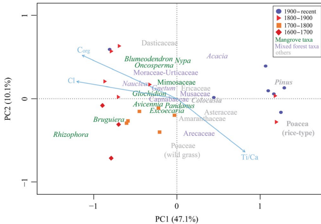
FIGURE 6 Principal component analysis (PCA) 1 and 2 for pollen data of the Segara Anakan Lagoon core. The mangrove taxa and its associates are in green, while mixed forest and other taxa are in purple and gray, respectively. The vectors for C accumulation, C_{org} (%), Ti/Ca and seawater/salt elements (Cl) are represented by blue arrows radiating from the center
