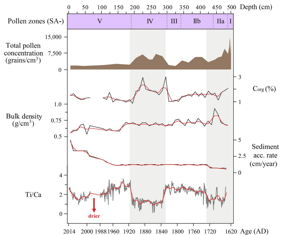
FIGURE 5 Total pollen concentration, \text{C}_{\text{org}} content, bulk density, and sediment accumulation rate of the Segara Anakan Lagoon core. The gray bars highlight the periods of lower precipitation in the Segara Anakan and its catchment area as indicated by \text{Ti}/\text{Ca}
