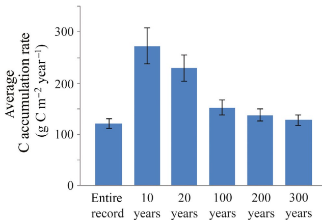
FIGURE 7 Average C accumulation rate for the SAL in different time slices
