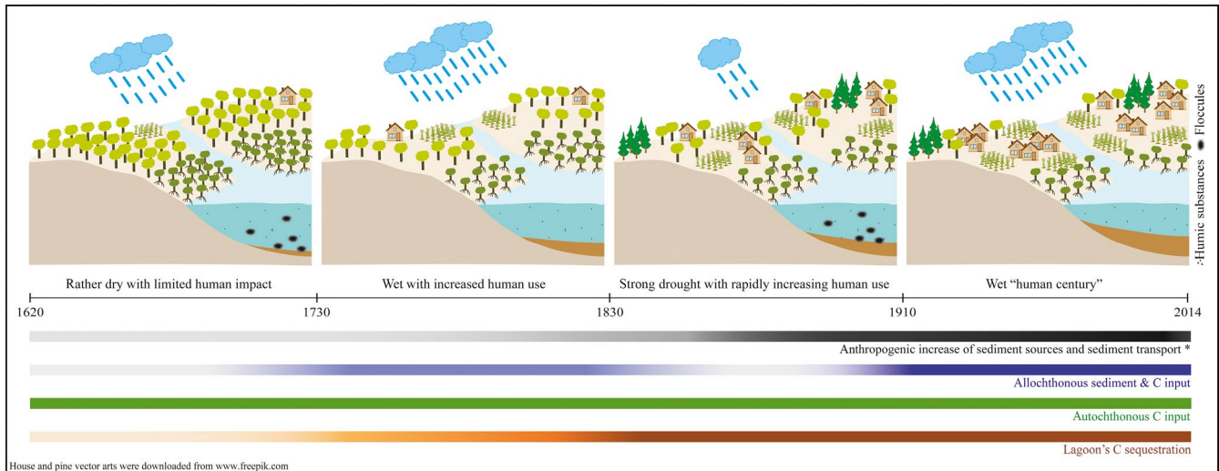
FIGURE 9 Four phases of environmental development of the SAL as controlled by the intertwined effects of climate and land use change. The division of the phases is based on the changes in precipitation in the Segara Anakan and its catchment area as indicated by Ti/Ca. (*more detailed information on the sediment sources is in Lukas, 2017)
