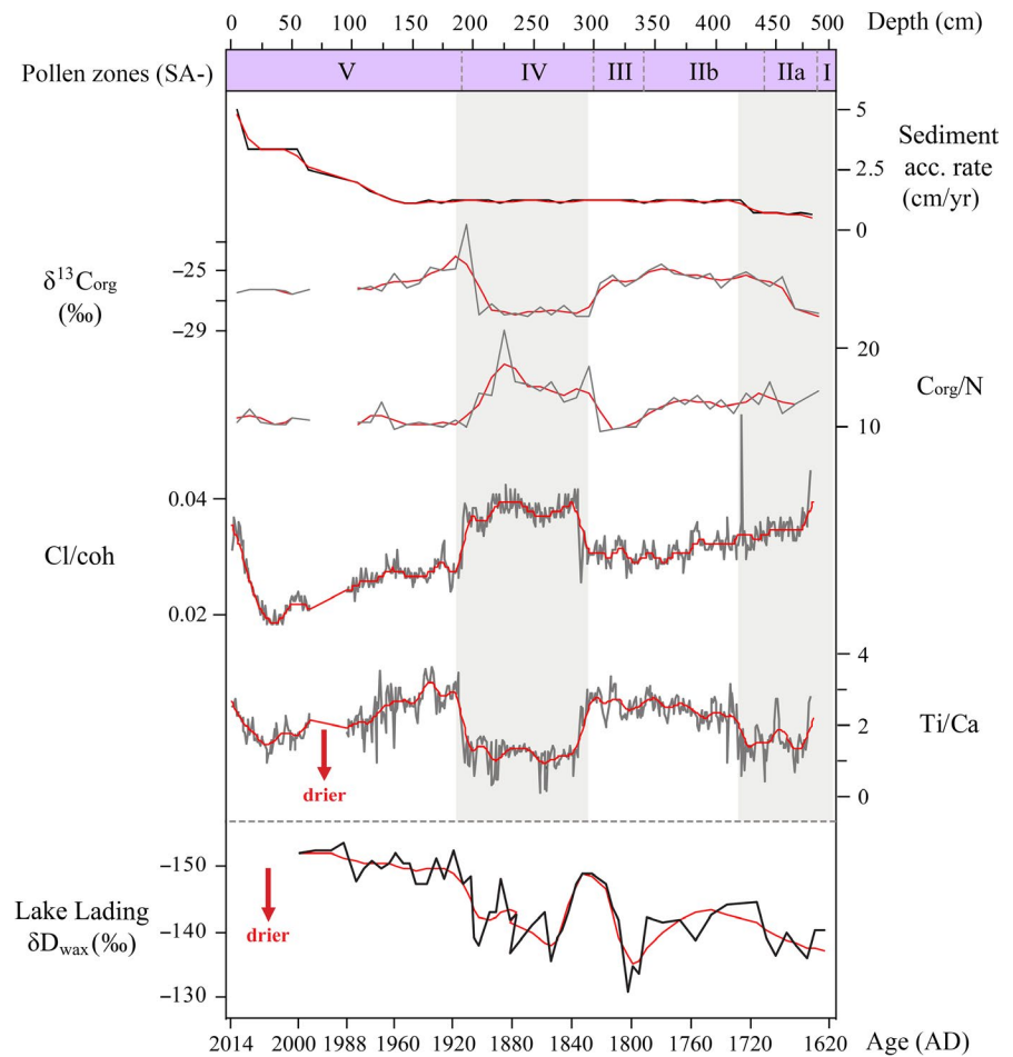
FIGURE 4 Records of sediment accumulation rate, \delta^{13}\text{C}_{\text{org}} , \text{C}_{\text{org}}/\text{N} , \text{Cl} , and \text{Ti}/\text{Ca} of the Segara Anakan Lagoon compared with the \delta\text{D}_{\text{wax}} record of Lake Lading in East Java (Konecky et al., 2003). The correlation between \text{Ti}/\text{Ca} from the SAL and \delta\text{D}_{\text{wax}} from Lake Lading is relatively strong and significant ( r = -.55 ; p\text{-value } 9.435\text{e-}06 ; Supplementary S5). The gray bars highlight the periods of lower precipitation in the Segara Anakan and its catchment area as indicated by the \text{Ti}/\text{Ca} ratio
